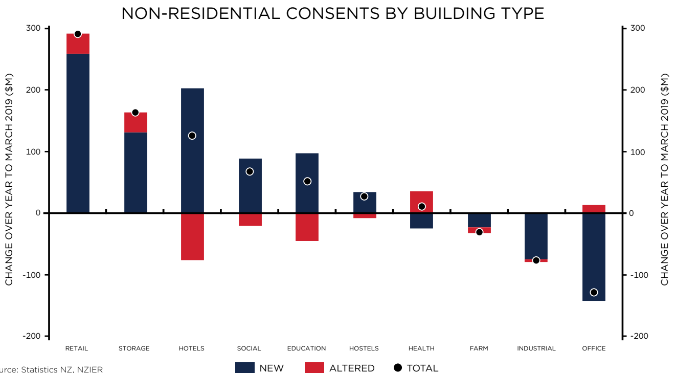
FIGURE 5 Retail demand remains top driver of growth in non-residential construction demand Annual change in consents, $m, year ended March 2019
